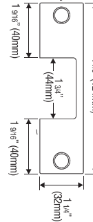
Latchbolt faceplate
